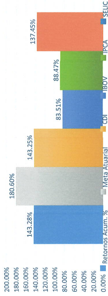
Benchmarking
